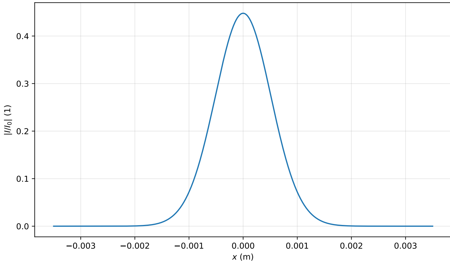
Intensity profile I(x, y = 0, z = 2.388m)/I_0 , P_{in}=0.1P_{cr} , artificial time
